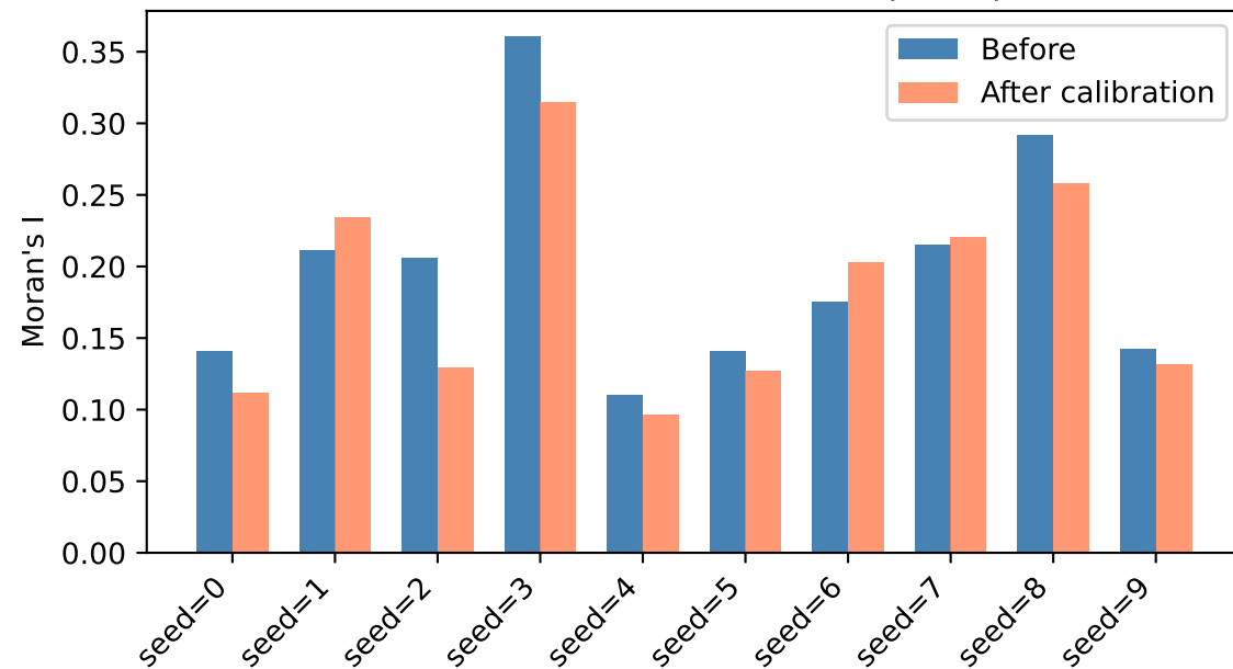
Moran's I: before vs after — ('compas', 'platt')
